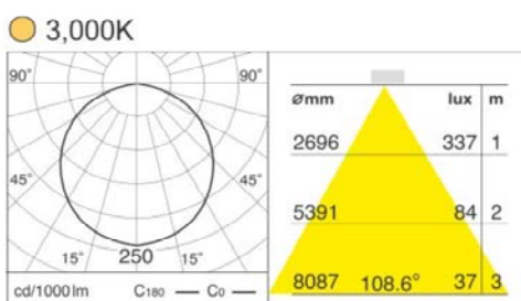
Photometrie
